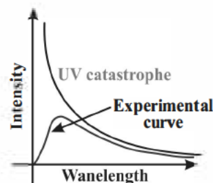
Figure 25.3 ultraviolet catastrophe
