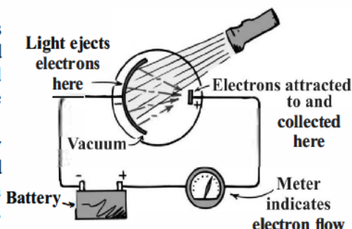
Figure 25.4 Photoelectric Effect
