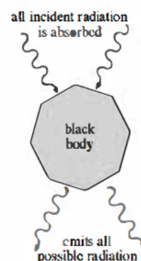
Figure 25.1 Black body Radiation
