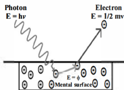
Figure 25.6 photo-electric effect
